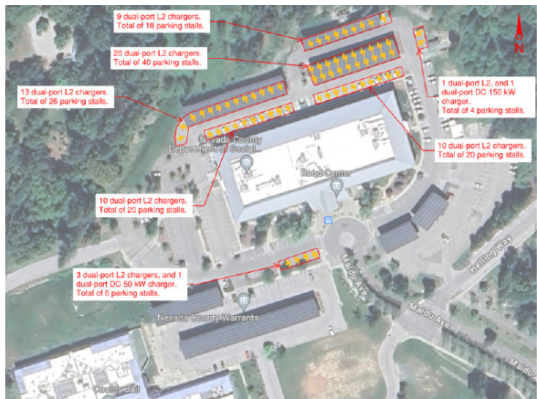
Figure 28: Recommended Charger Locations for ERAC
