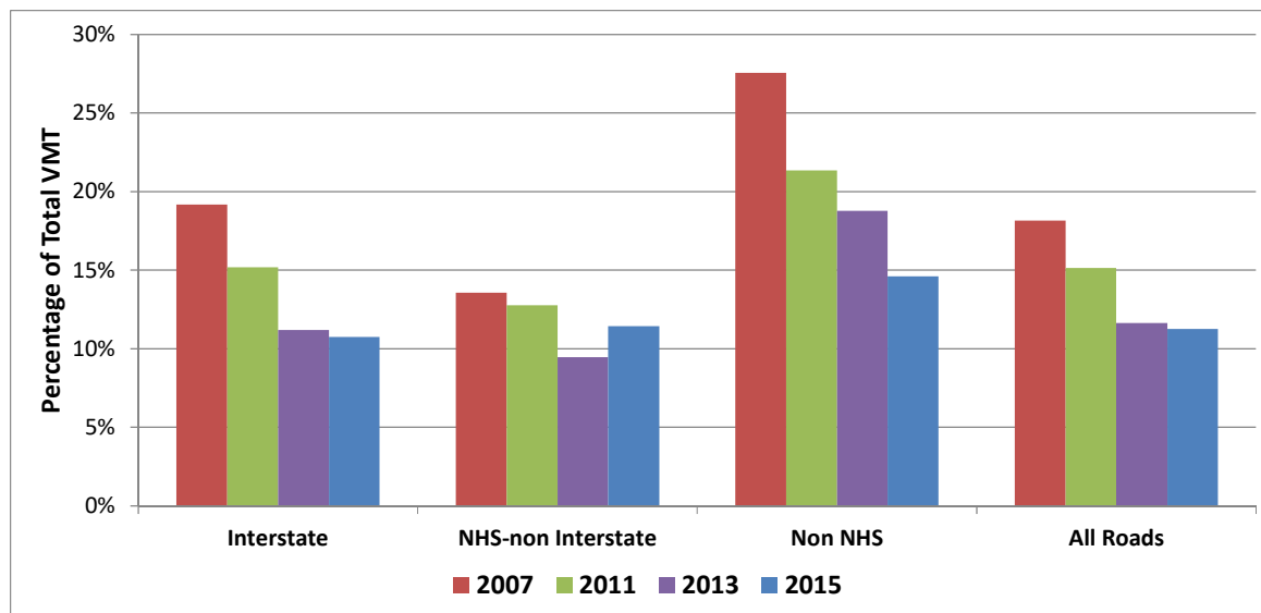
Figure 3. Poor Pavements by Total VMT (IRI > 170 inches per mile)
